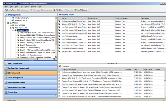
OS deployment in CapalInstaller Management Console.
